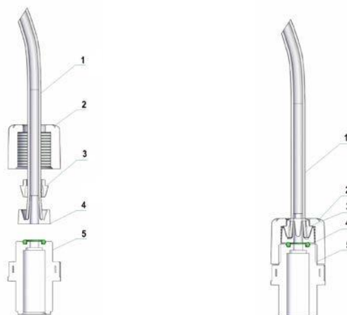
Fig.4 – Hydraulic Connection
