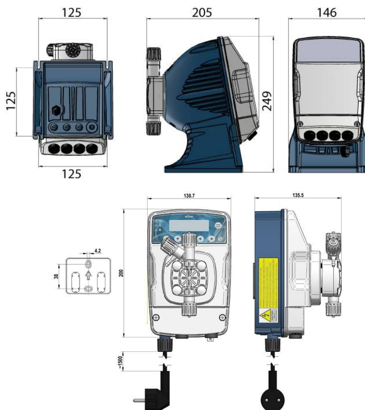
Fig. 1 - Pump and plate for wall mounting (dimensions in mm.)
